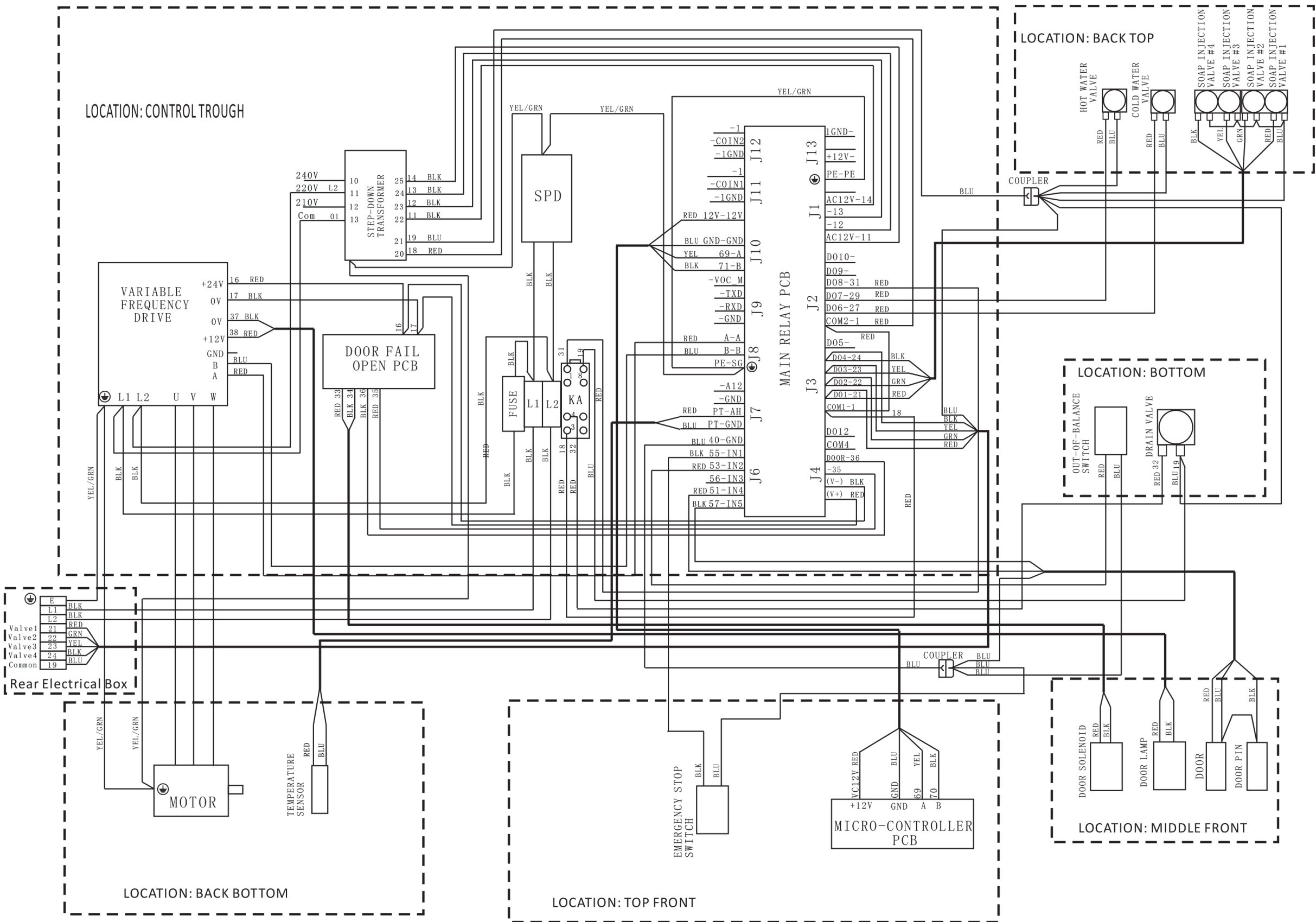
UNITY LAUNDRY SYSTEMS WASHER EXTRACTOR MODEL UTS29 WIRING SCHEMATIC - MICRO CONTROLLER VF DRIVE, 208-240V, 1PH, 50-60HZ
