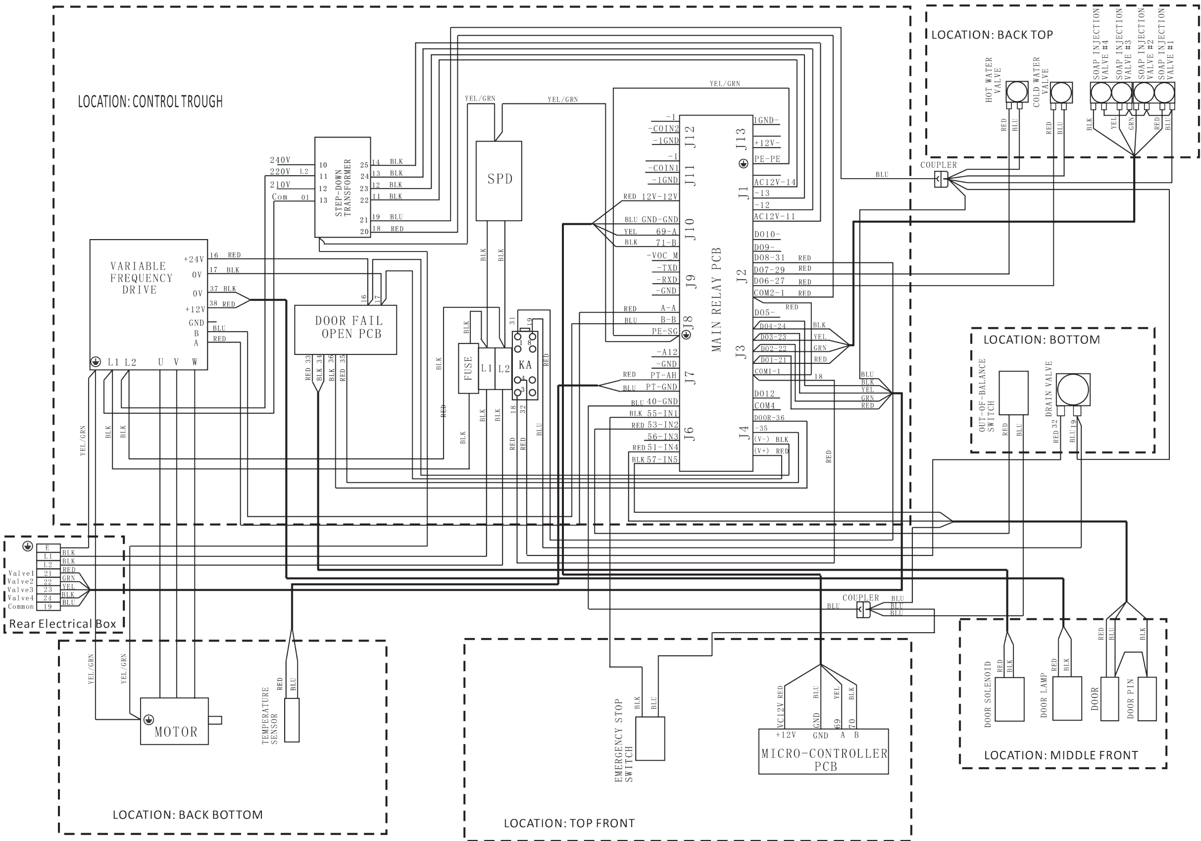
UNITY LAUNDRY SYSTEMS WASHER EXTRACTOR MODEL UTS40 /UTS62 WIRING SCHEMATIC - MICRO CONTROLLER VF DRIVE, 208-240V, 1PH, 50-60HZ
