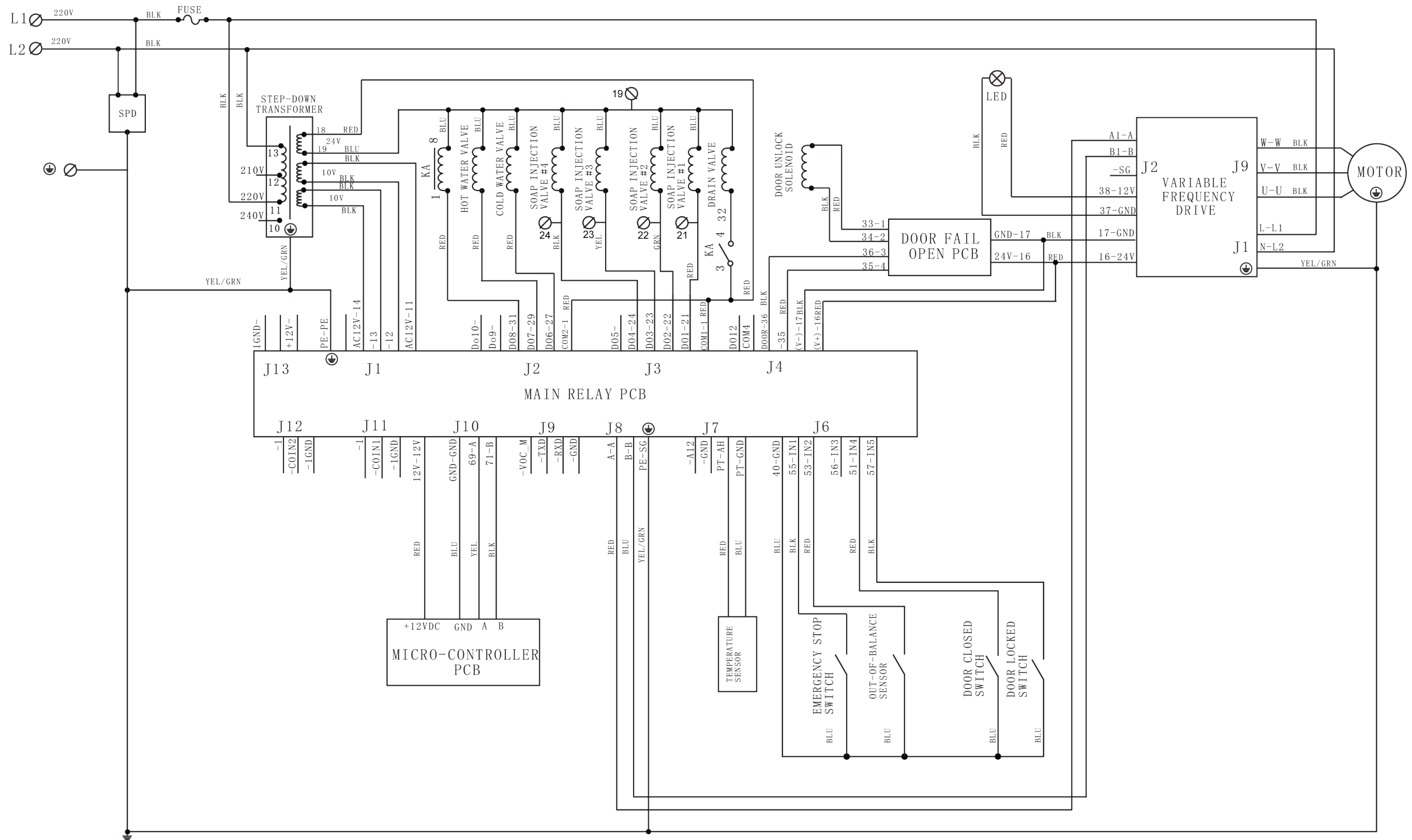
UNITY LAUNDRY SYSTEMS WASHER EXTRACTOR MODEL UTS40 / UTS62 WIRING SCHEMATIC VF DRIVE, 208-240V, 1PH, 50-60HZ
