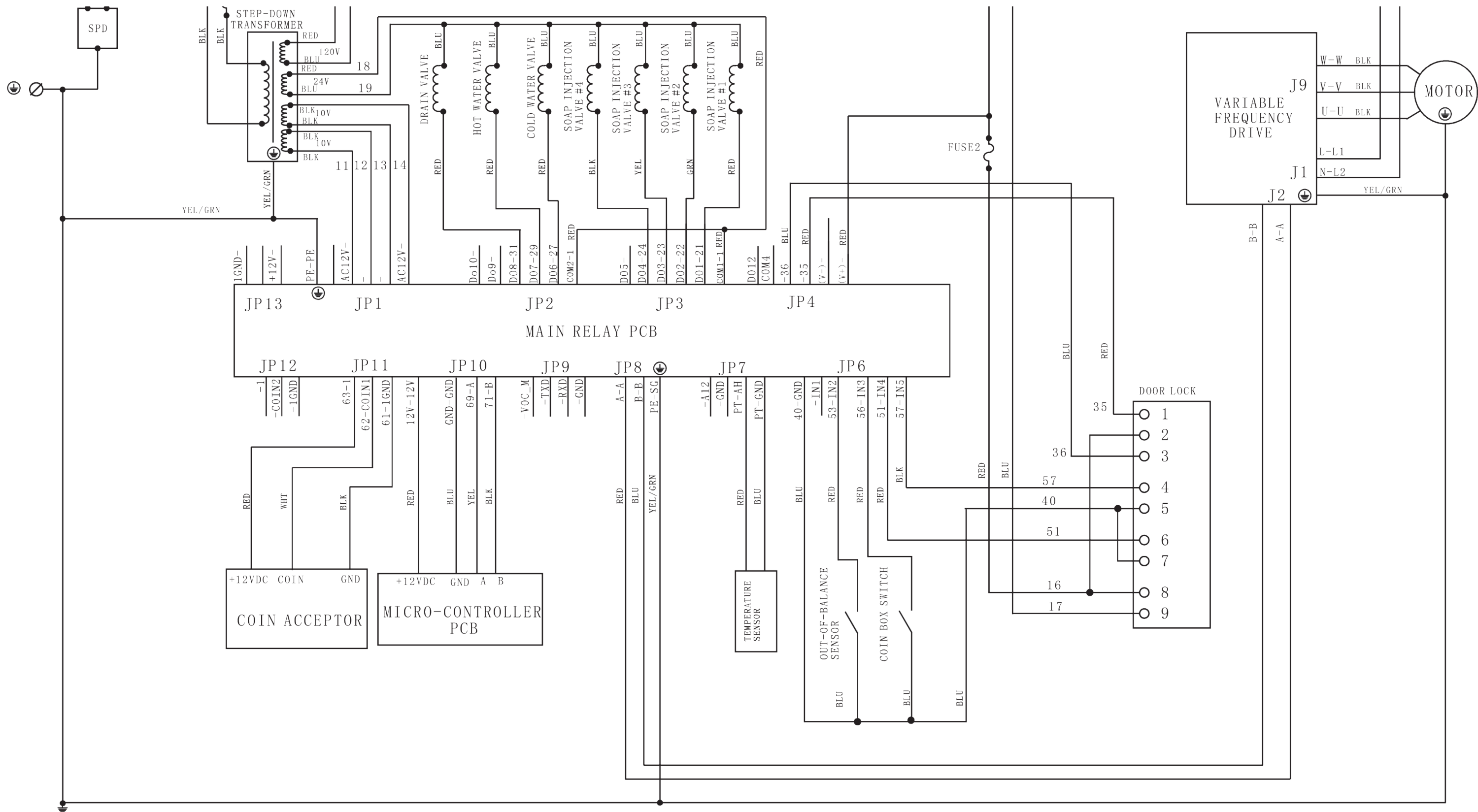
UNITY LAUNDRY SYSTEMS WASHER EXTRACTOR MODEL UTS29 WIRING SCHEMATIC VF DRIVE, 208-240V, 1PH, 50-60HZ
